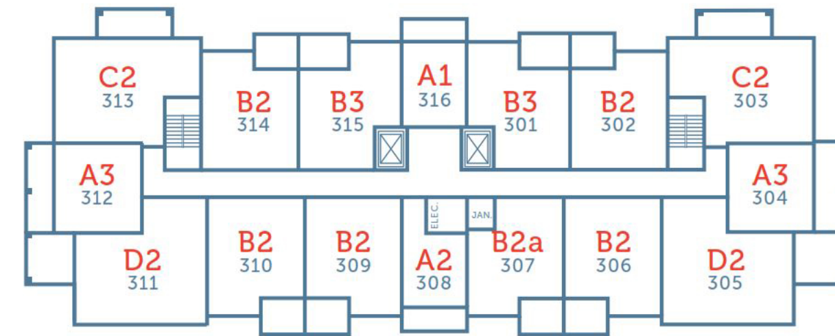
FLOOR 3
